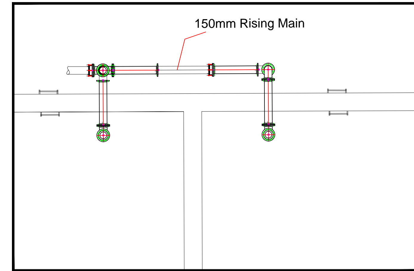
PLAN OF INLET DETAIL Scale @ A1 1/50 A3 1/100
