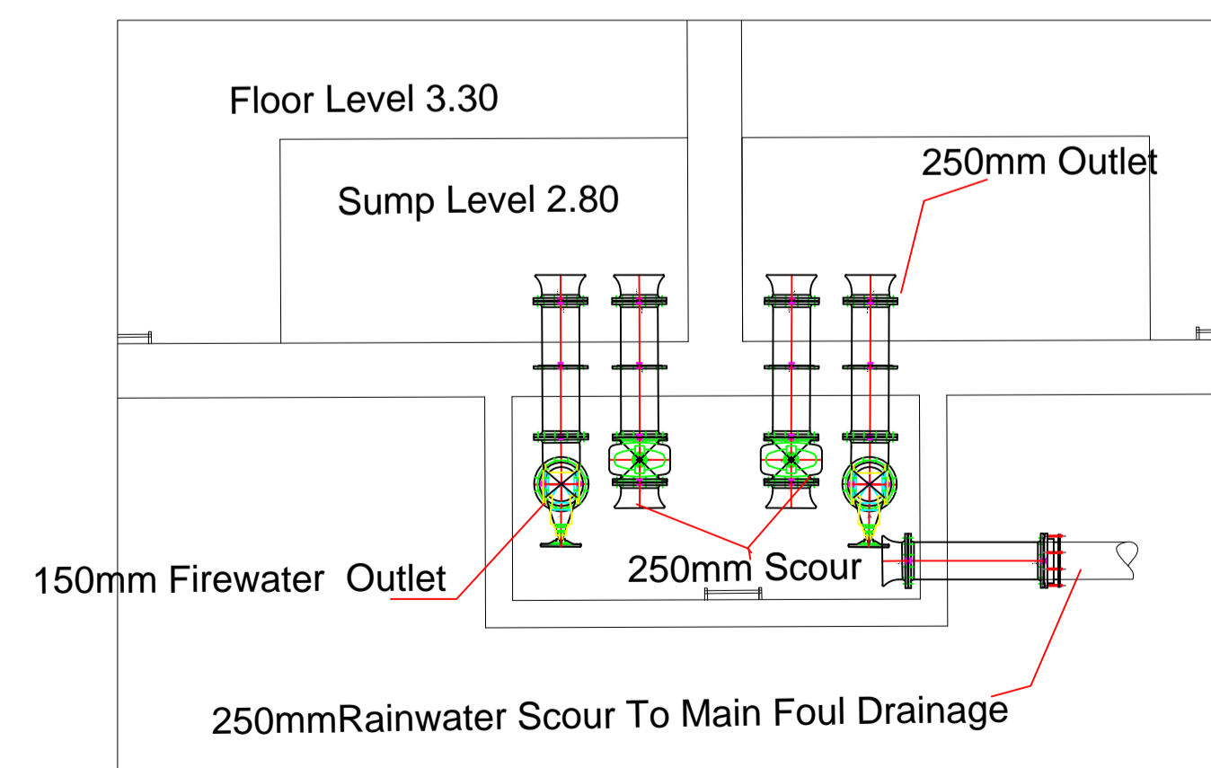
PLAN OF OUTLET DETAIL Scale @ A1 1/50 A3 1/100
